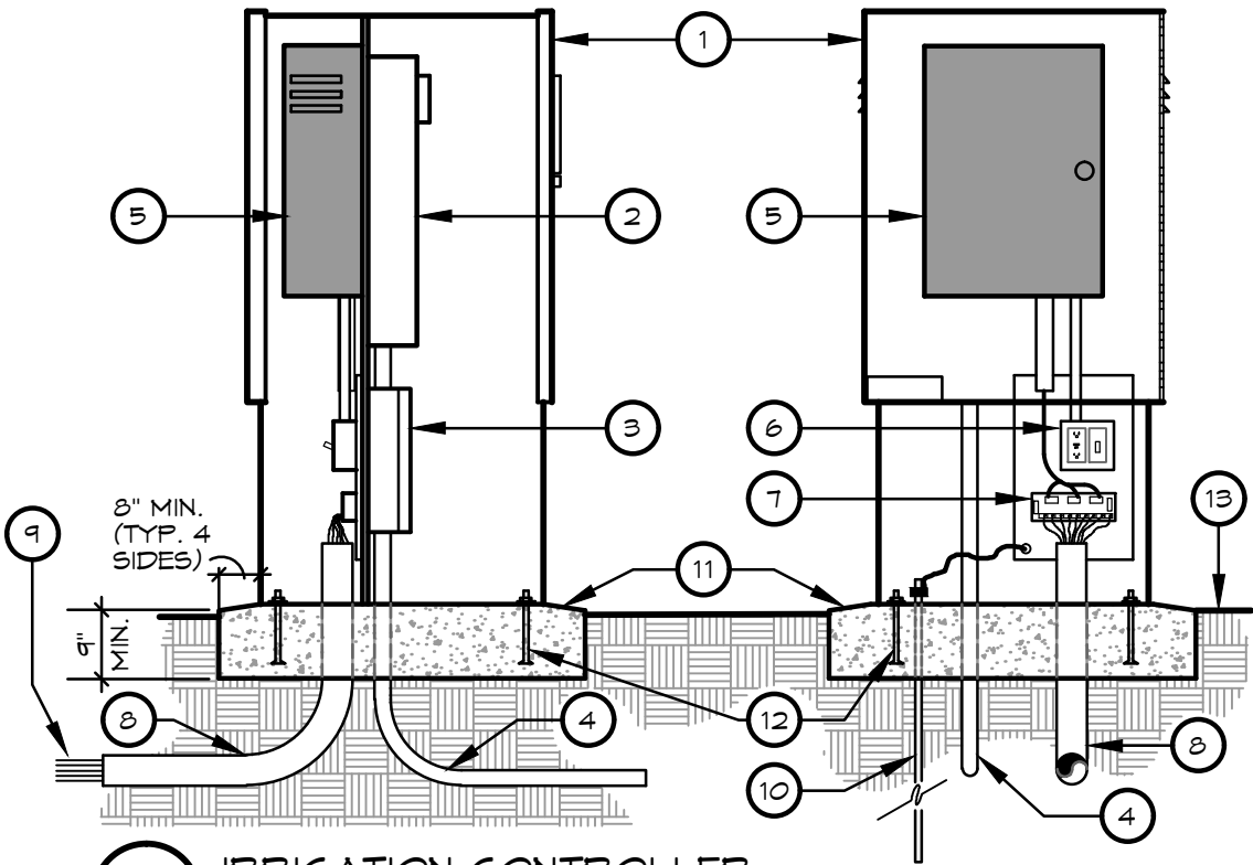
SIDE VIEW
